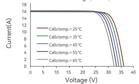
Current-Voltage(455W)
